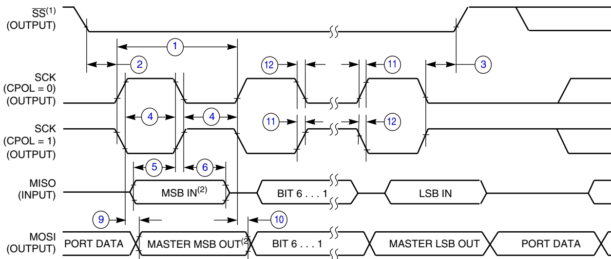
Figure A-17. SPI Master Timing (CPHA = 0)
