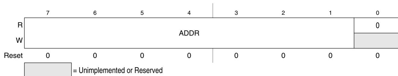
Figure 13-3. IIC Address Register (IICA)
