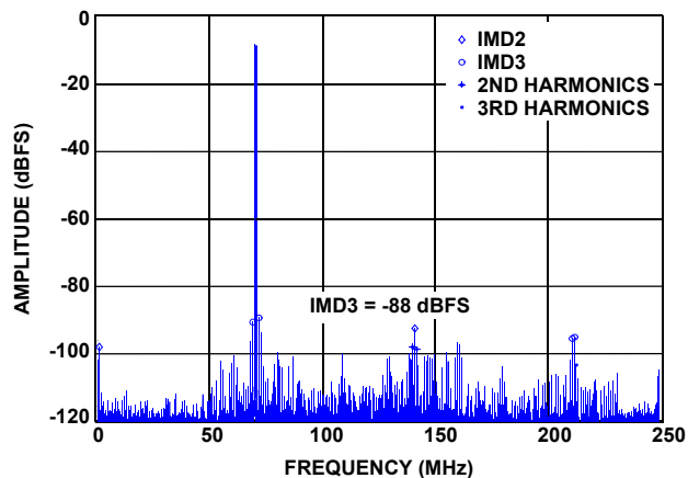
FIGURE 16. TWO-TONE SPECTRUM (F1 = 70MHz, F2 = 71MHz -7dBFS)
