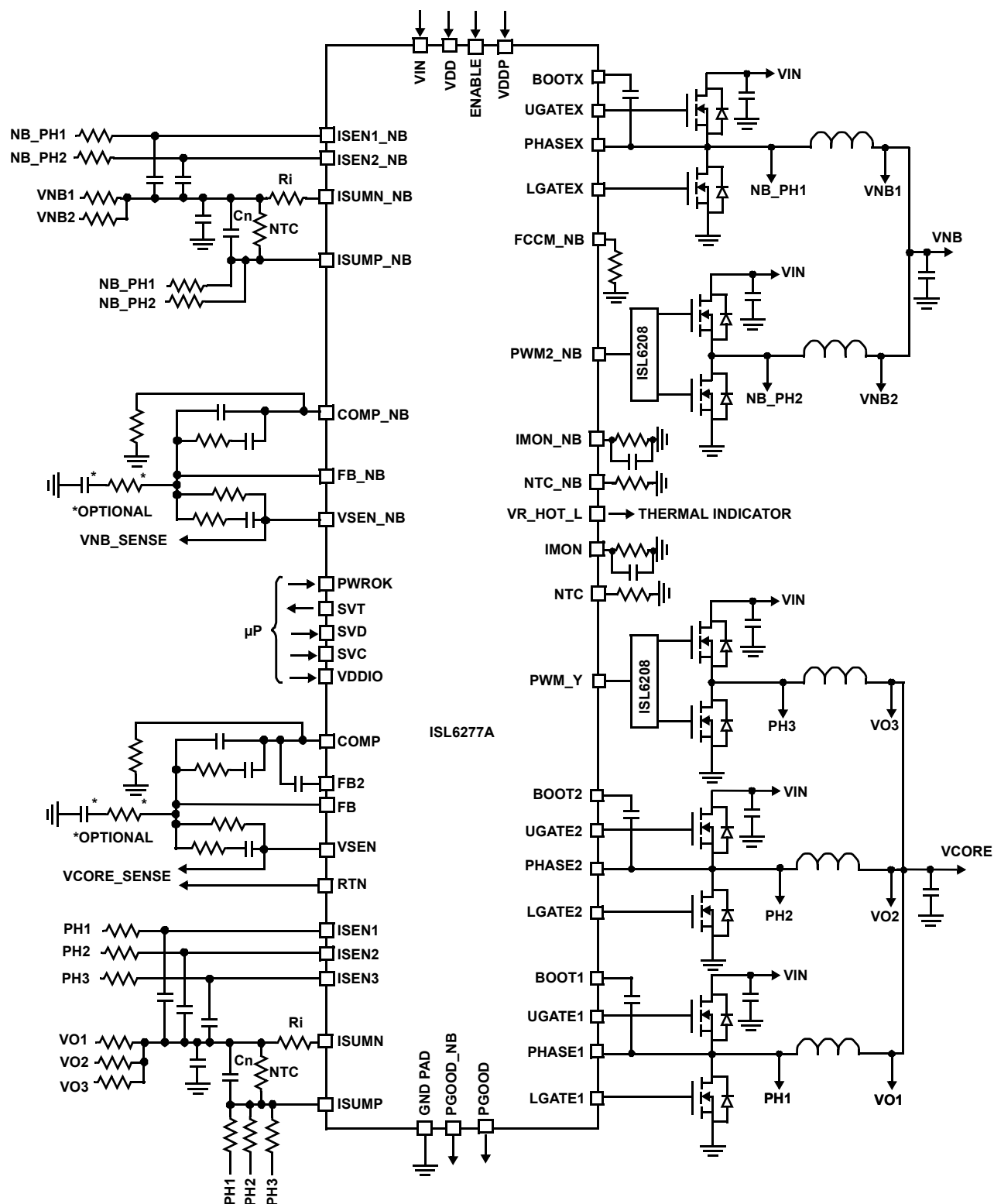
FIGURE 3. TYPICAL APPLICATION CIRCUIT USING INDUCTOR DCR SENSING
