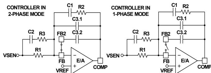
FIGURE 20. FB2 FUNCTION
