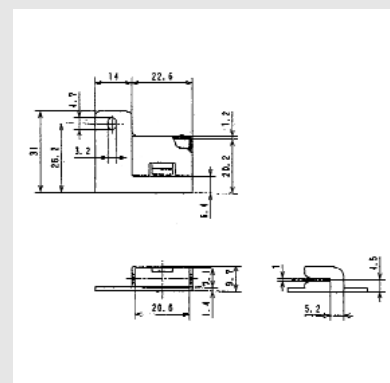
Part No.: FRHL-20 Material: PA66 UL94V-2
