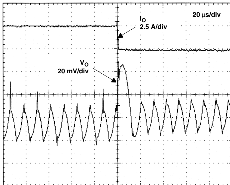
Figure 28. Falling Load Transient Response
