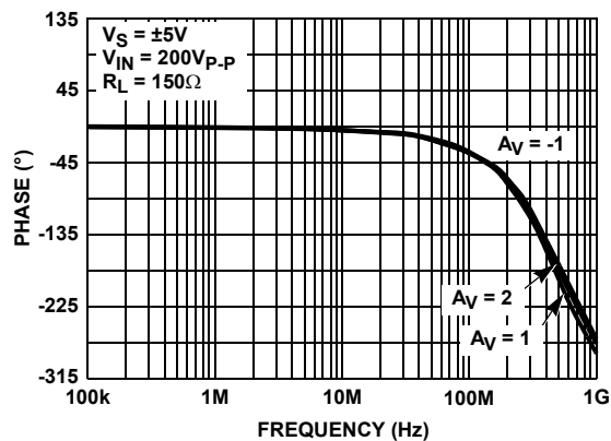
FIGURE 2. PHASE RESPONSE
