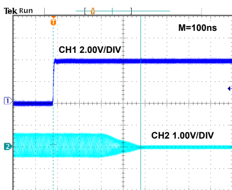
FIGURE 17. DISABLED RESPONSE
