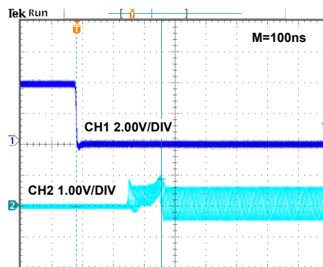
FIGURE 18. ENABLED RESPONSE
