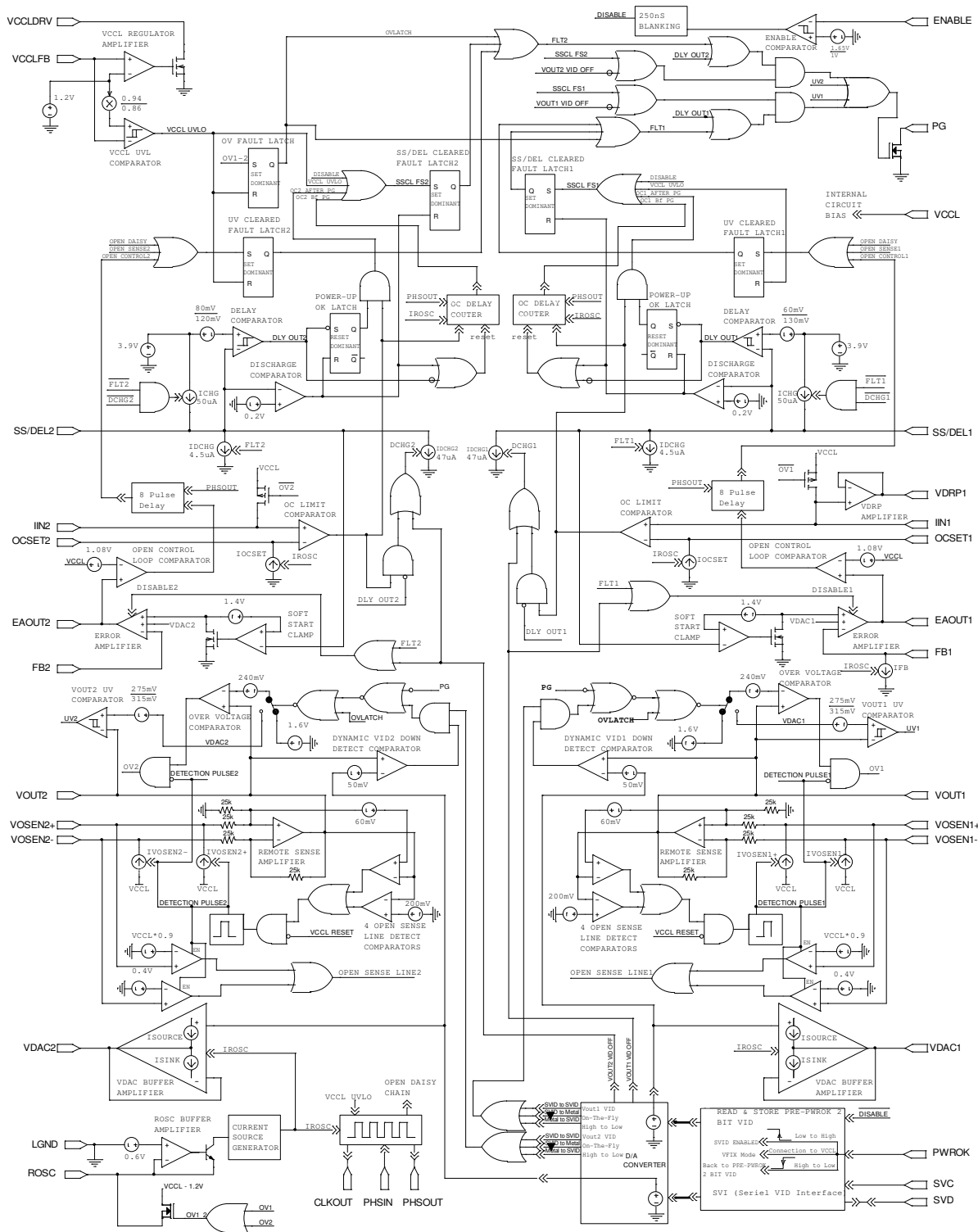
Figure 8 Block Diagram
