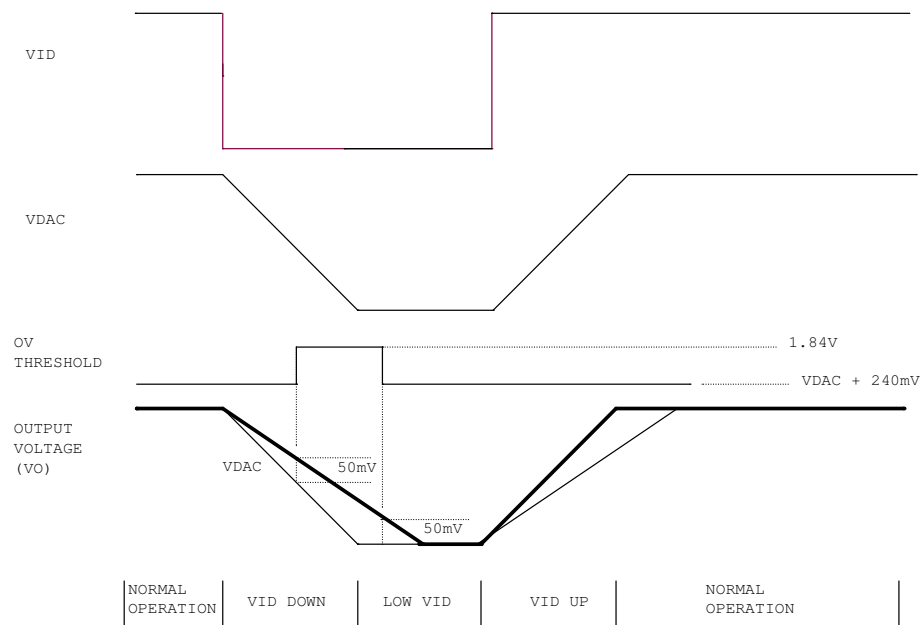
Figure 16 Over-voltage protection during dynamic VID
