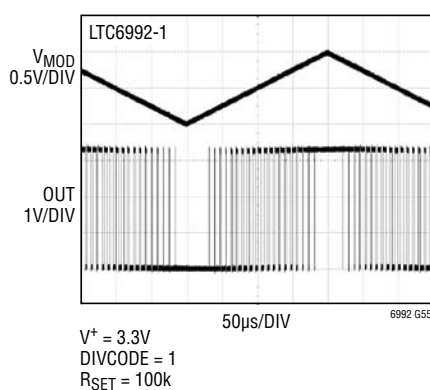
125kHz Full Modulation
