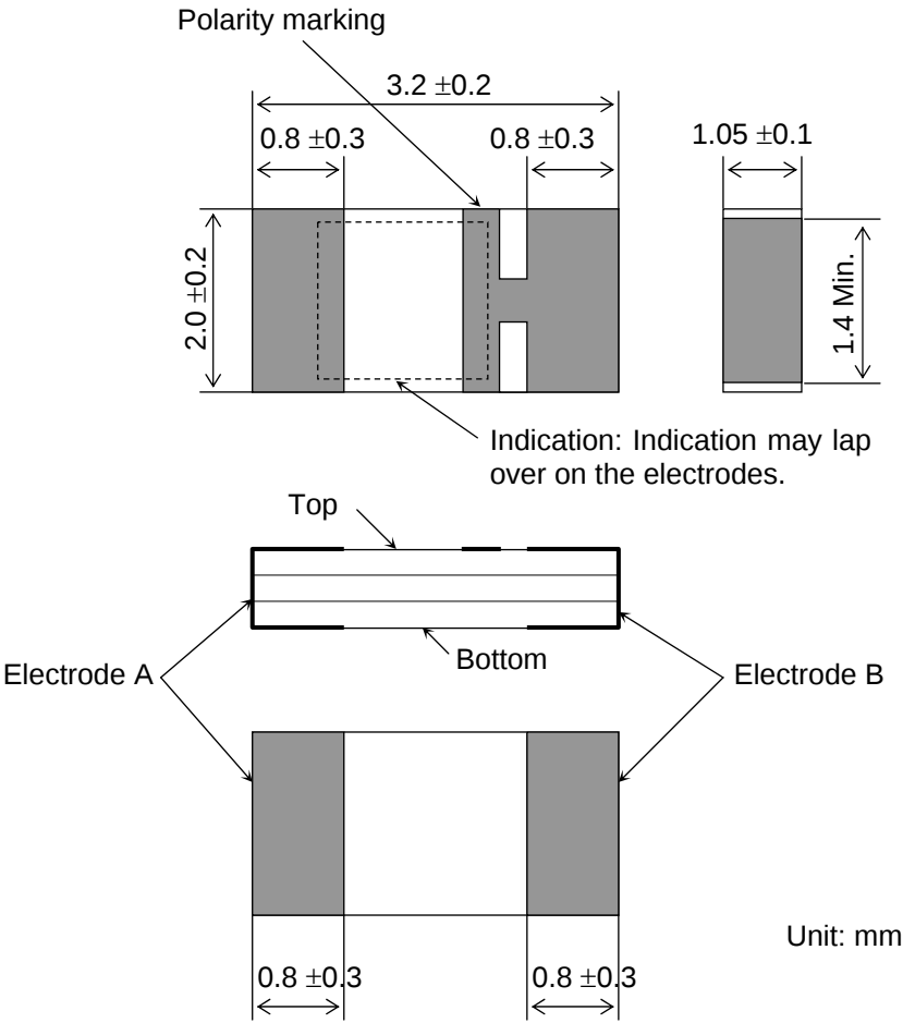
Figure 2. Dimensions
