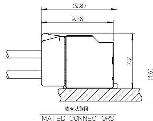
MATED CONNECTORS
