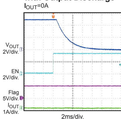
Turn Off Delay and Fall Time with Output Discharge I_{OUT} = 0A
