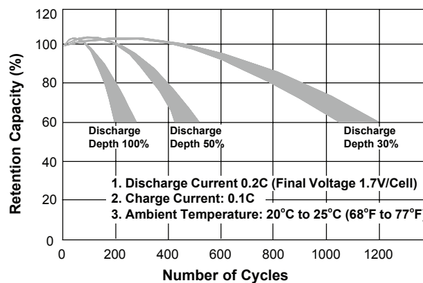
Life Characteristics in Cyclic Use
