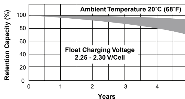
Life Characteristics in Stand-By Use
