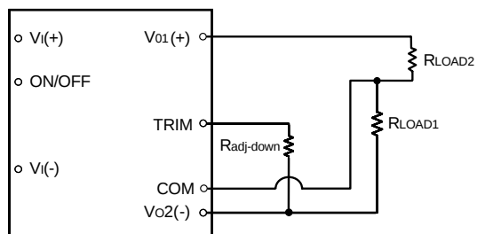
Figure 6. QW030-Series Circuit Configuration to Decrease Output Voltage
