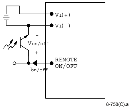
Figure 4. QW030-Series Remote On/Off Implementation
