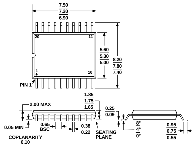
Figure 27. 20-Lead Shrink Small Outline Package [SSOP] (RS-20)
