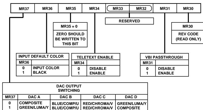
Figure 42. Mode Register 3
