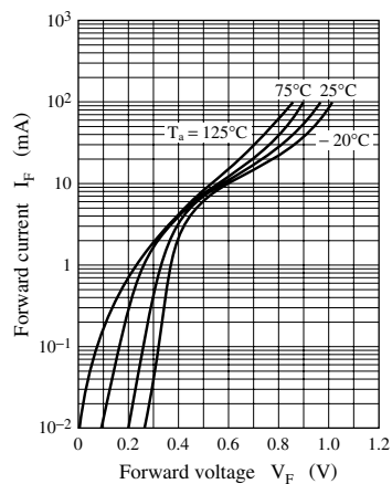
I_F - V_F (Between pins 1 and 4, 2 and 3)
