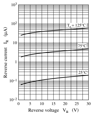
I_R - V_R (Between pins 1 and 4, 2 and 3)
