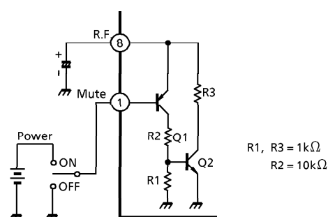
Fig.4 Mute circuit
