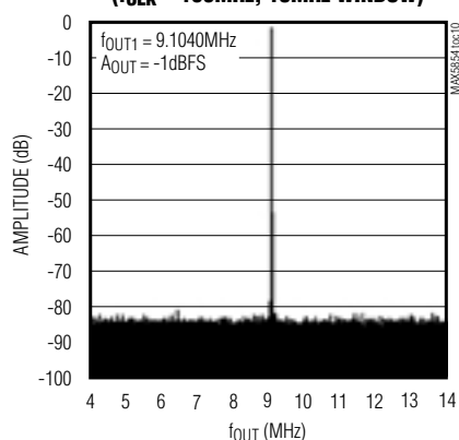
SINGLE-TONE SFDR ( f_{CLK} = 165MHz , 10MHz WINDOW)
