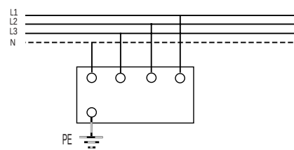
TT - TNS - IT networks
