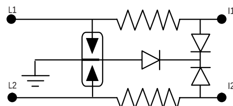
Series protection
