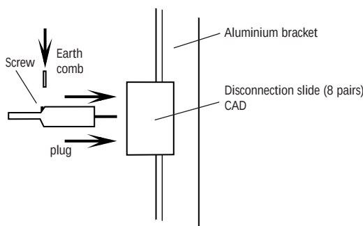
Module connection
