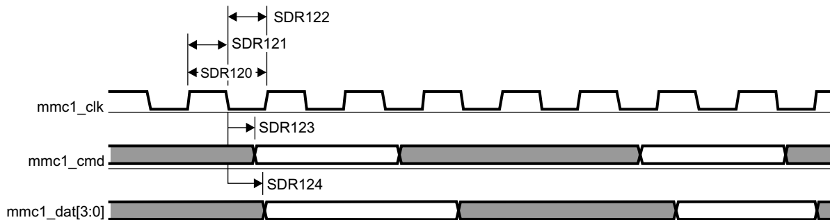
Figure 5-78. MMC/SD/SDIO in - High Speed SDR12 - Transmitter Mode
