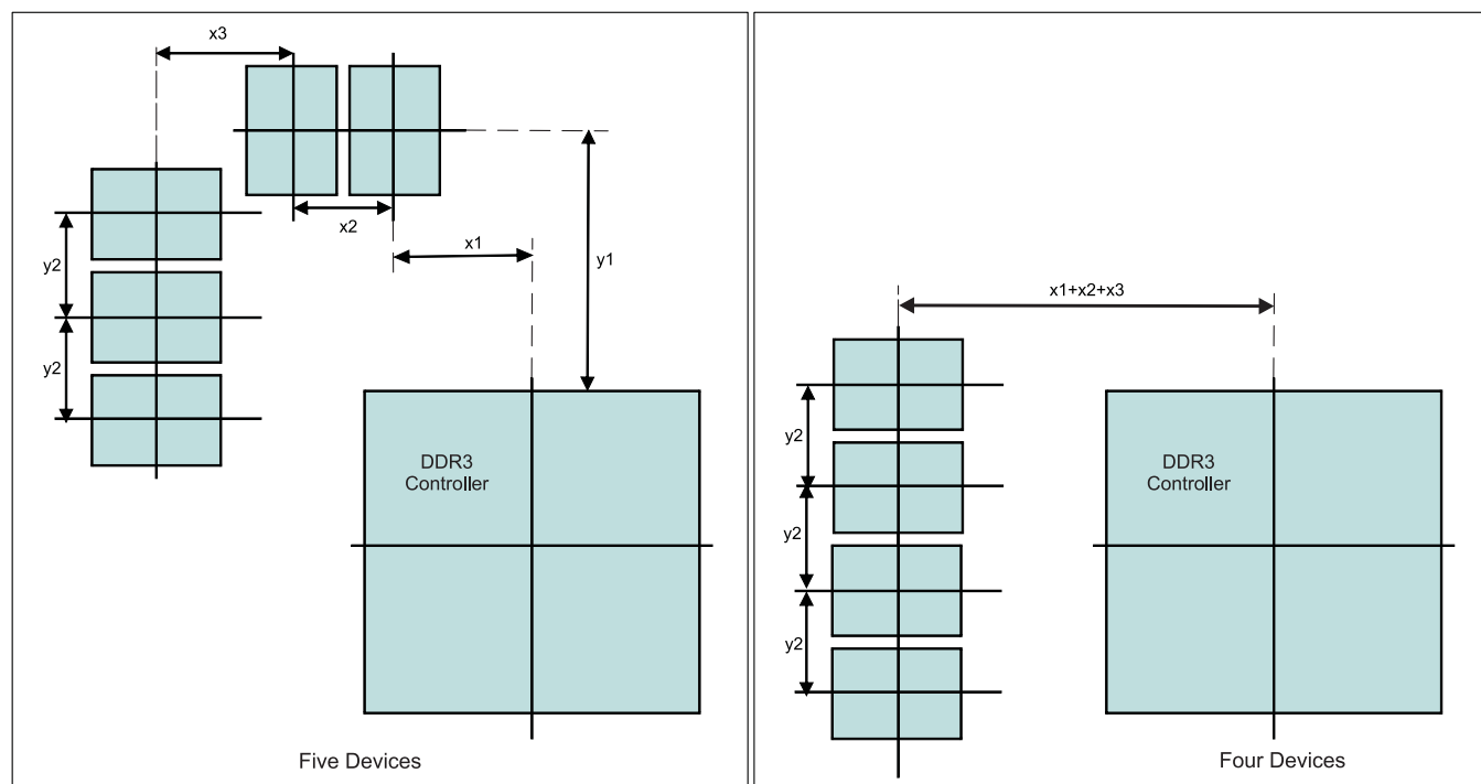
Figure 7-4. Placement Specifications
