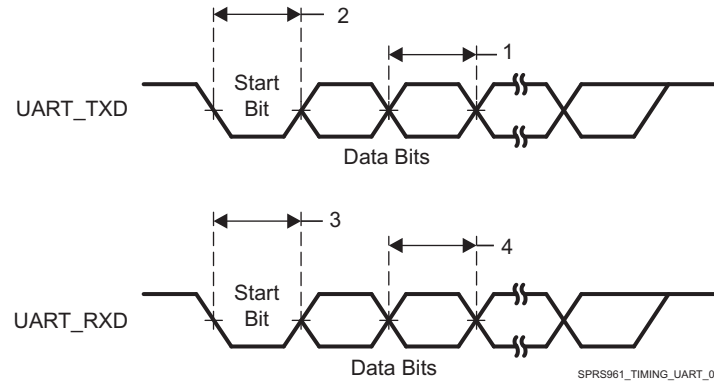
Figure 5-45. UART Timing
