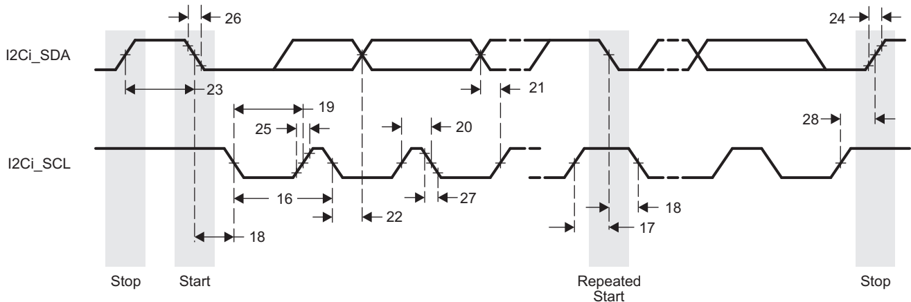
Figure 5-37. I2C Transmit Timing
