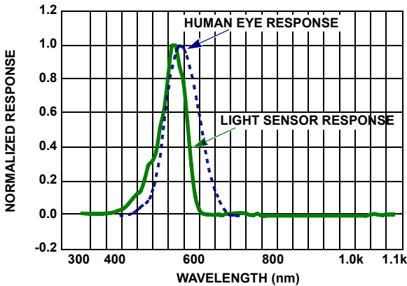
FIGURE 3. SPECTRAL RESPONSE
