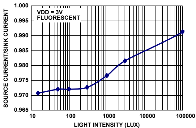
FIGURE 10. RATIO OF SOURCE CURRENT AND SINK CURRENT vs LIGHT INTENSITY
