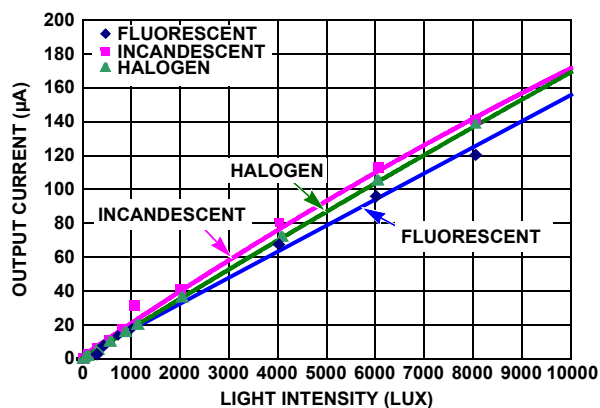
FIGURE 7. OUTPUT CURRENT vs LIGHT INTENSITY
