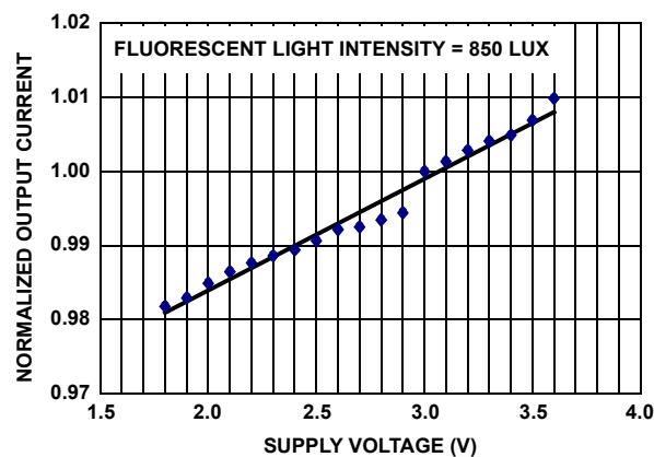
FIGURE 16. NORMALIZED OUTPUT CURRENT vs SUPPLY VOLTAGE
