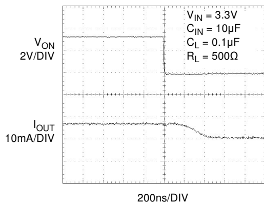
Figure 19. T_{OFF} Response
