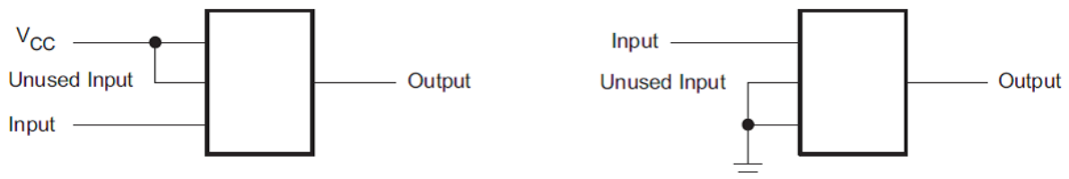
Figure 7-1. Layout Example
