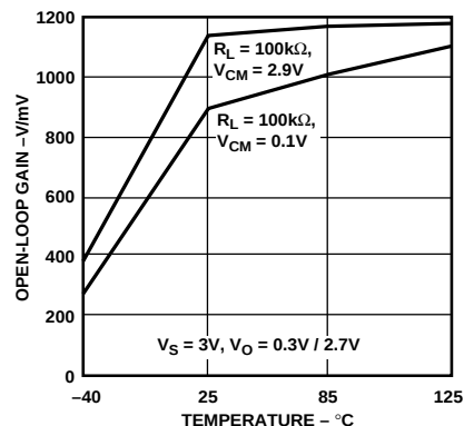
Figure 10. Open-Loop Gain vs. Temperature, V_S = +3\text{ V}
