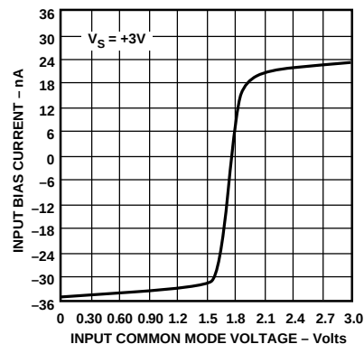
Figure 7. Input Bias Current vs. Common-Mode Voltage, V_S = +3\text{ V}
