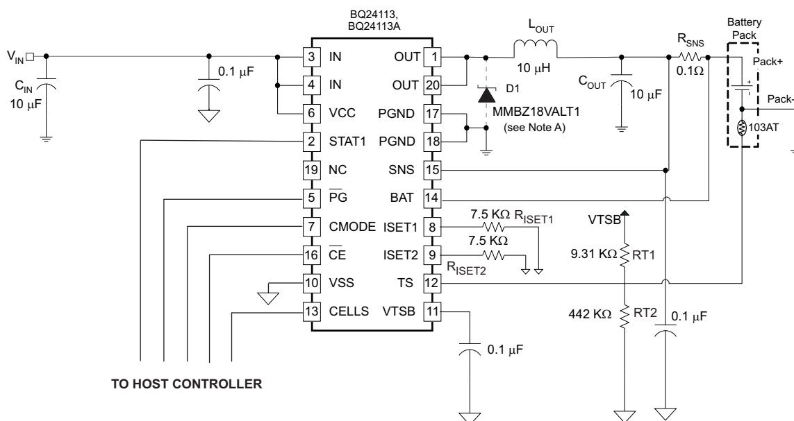
Figure 4. System-Controlled Application
