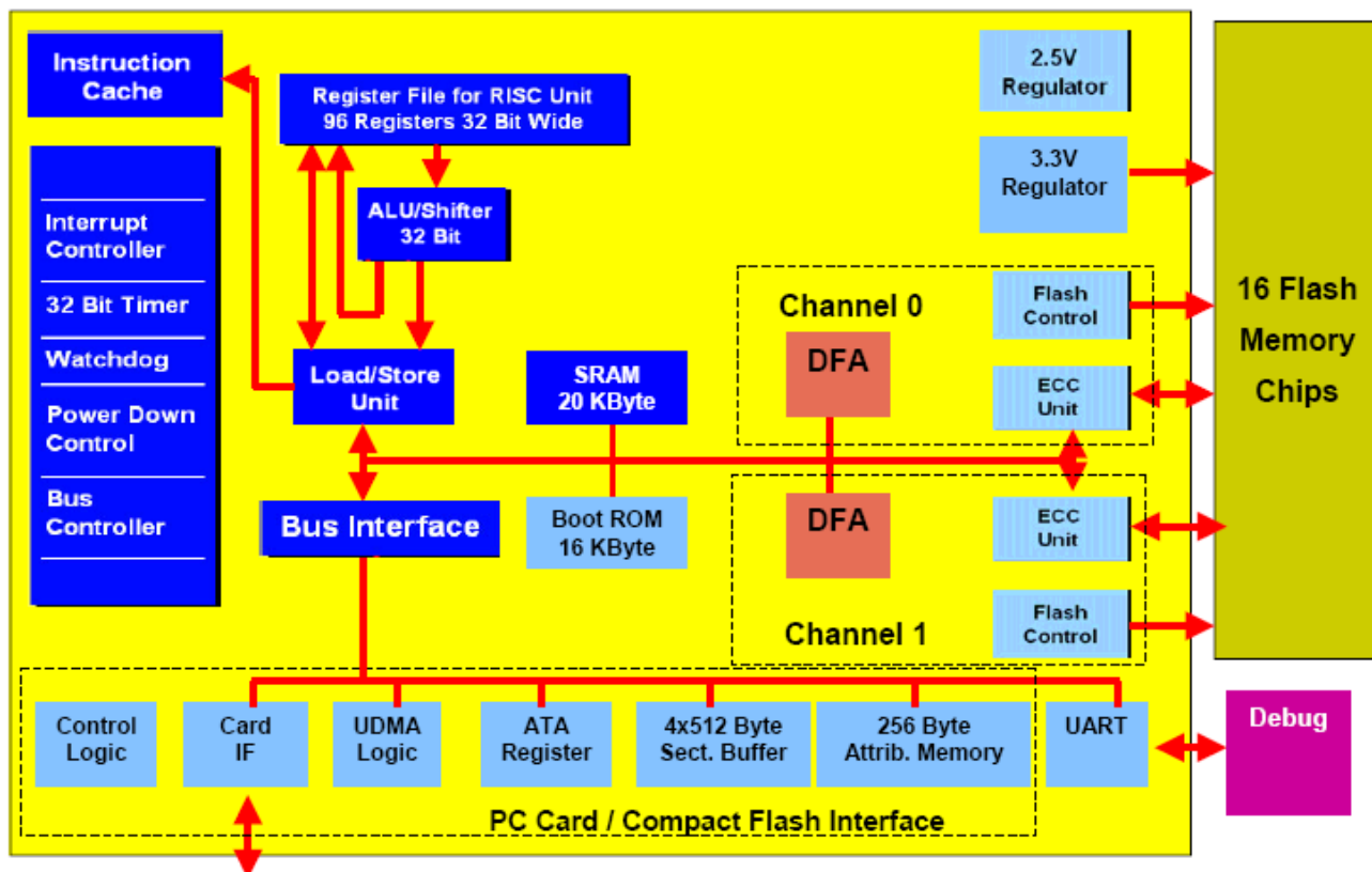
Figure 1-1: Block Diagram
