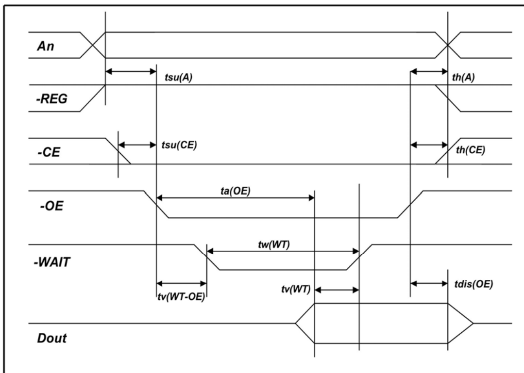
Figure 3-3: Common Memory Read Timing Diagram
