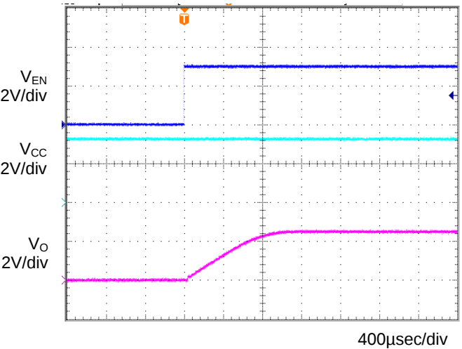
Figure 17. Input sequence 2 Co=1µF, Ta=105°C
