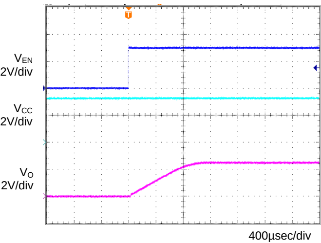
Figure 15. Input sequence 2 Co=1µF, Ta=-40°C
