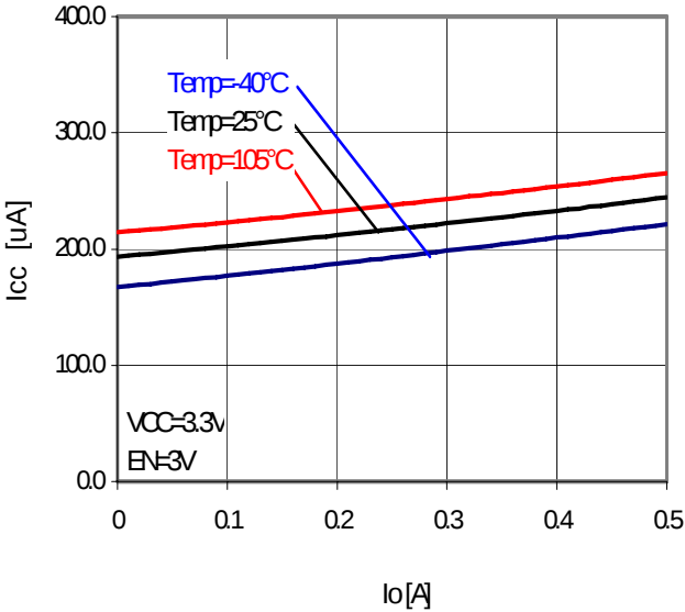
Figure 30. I_O-I_{CC}
