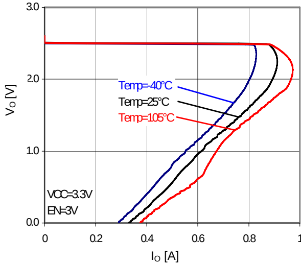
Figure 29. OCP
