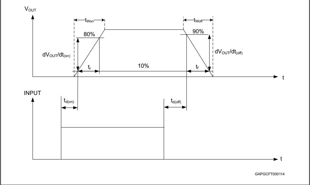
Figure 6. Switching characteristics
