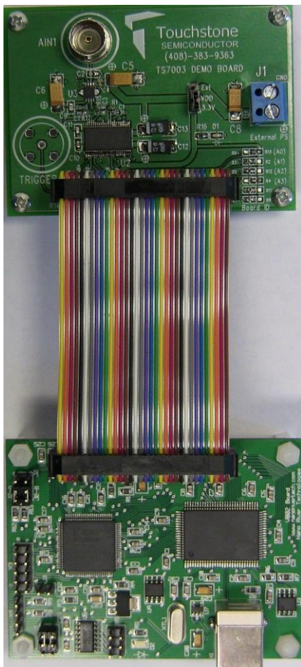
Figure 1. TS7003 Evaluation Board with Viperboard
