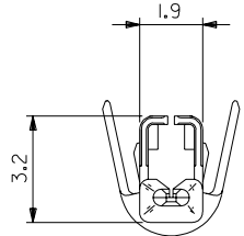
SECT. X-X
