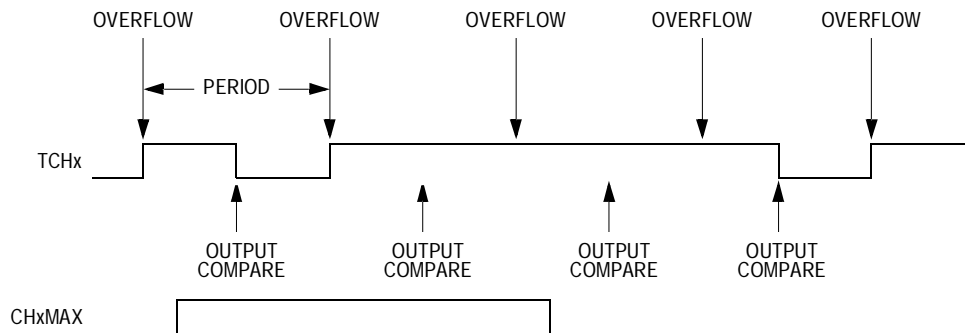
Figure 10-8. CHxMAX Latency
