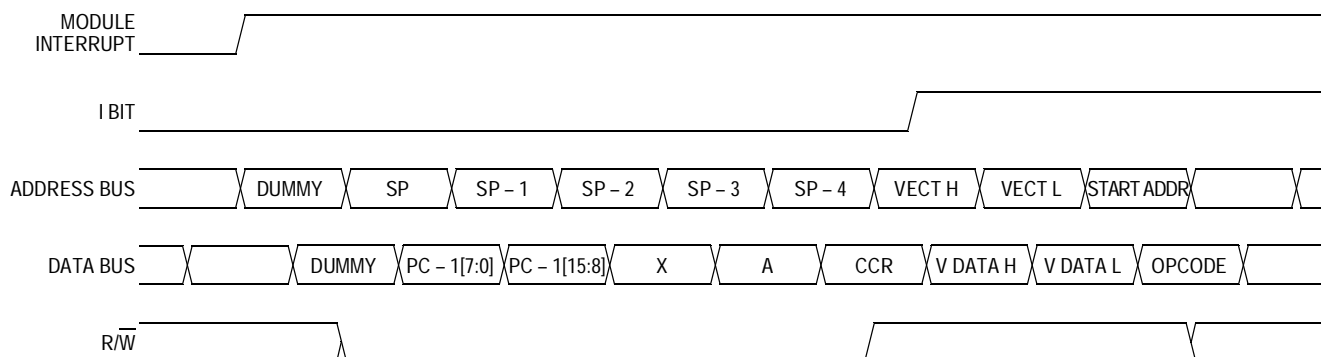
Figure 7-9. Interrupt Entry
