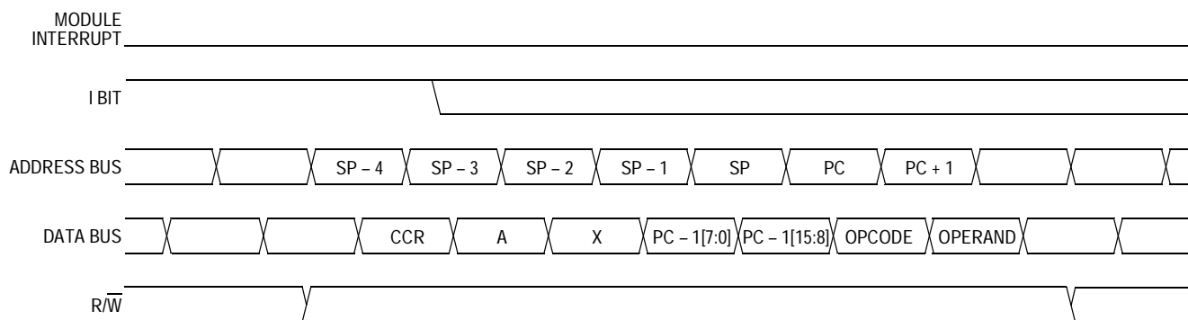
Figure 7-10. Interrupt Recovery
