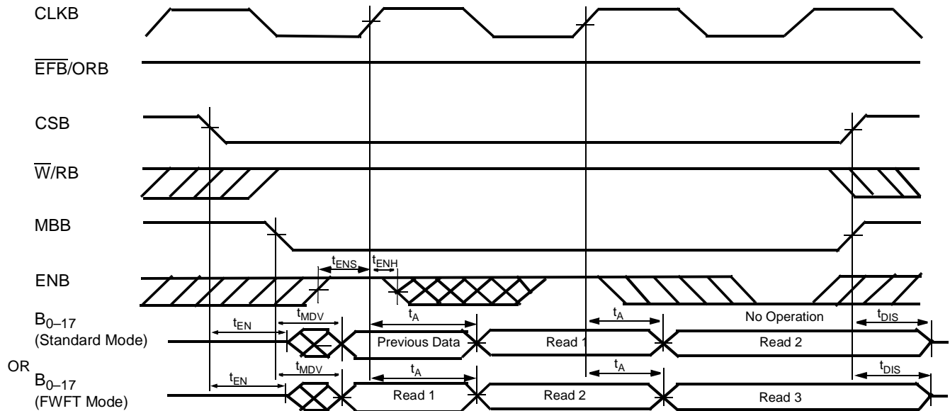
Port B Byte Read Cycle Timing for FIFO1 (CY Standard and FWFT Modes) [23]
