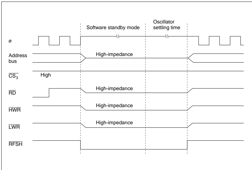
Figure 7-16 Signal Output Timing in Self-Refresh Mode (PSRAME = 1, DRAIME = 0)
