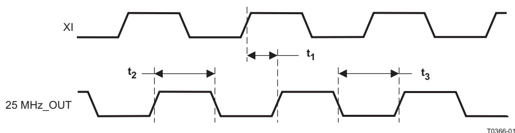
Figure 9-24. 25 MHz_OUT Timing
