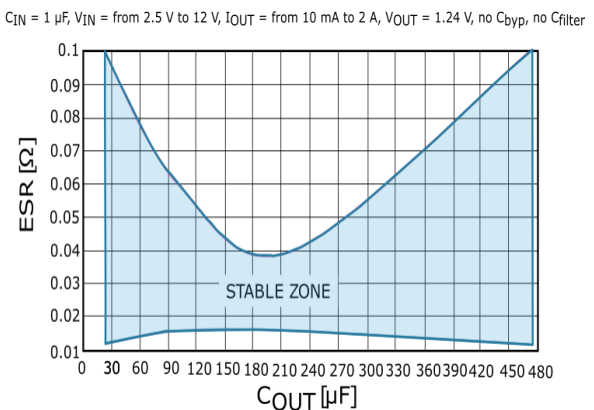
Figure 28: Stability area for tantalum capacitor
