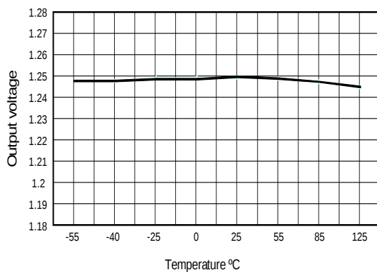
Figure 7: Output voltage vs temperature ( V_{IN} = 2.5\ \text{V} , I_{OUT} = 1\ \text{A} )
