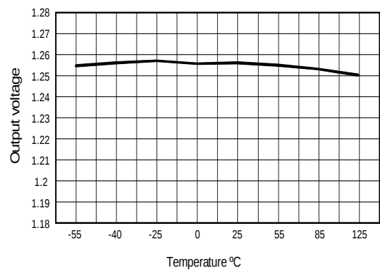
Figure 8: Output voltage vs temperature ( V_{IN} = 2.5\ \text{V} , I_{OUT} = 2\ \text{A} )
