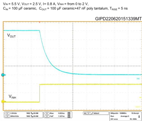
Figure 23: Turn-off transient
