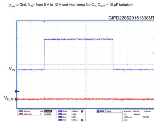
Figure 24: Line transient ( I_{OUT} = 0.8\text{ A} , V_{OUT} = 3\text{ V} )
