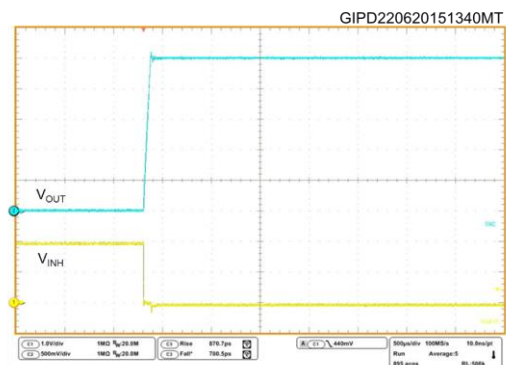
Figure 22: Turn-on transient
