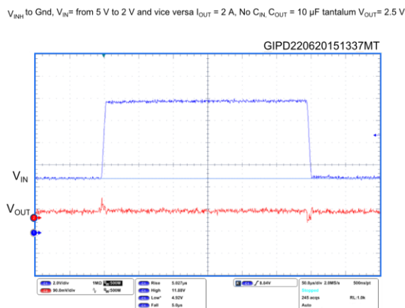
Figure 25: Line transient ( I_{OUT} = 2\text{ A} , V_{OUT} = 2.5\text{ V} )
