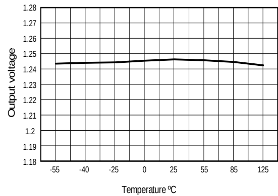
Figure 6: Output voltage vs temperature ( V_{IN} = 2.5\ \text{V} , I_{OUT} = 400\ \text{mA} )
