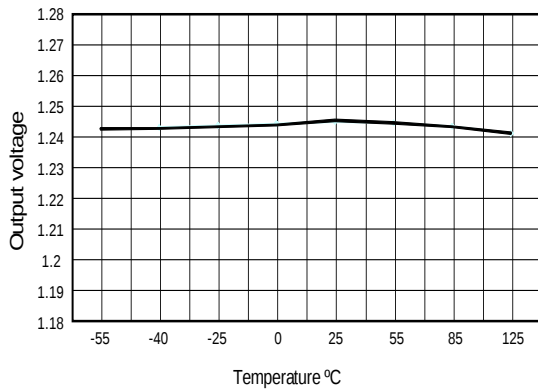
Figure 5: Output voltage vs temperature ( V_{IN} = 2.5\ \text{V} , I_{OUT} = 5\ \text{mA} )
