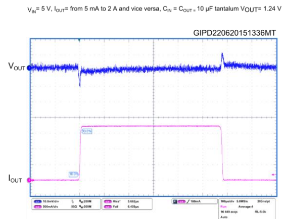
Figure 26: Load transient
