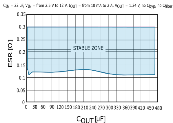
Figure 27: Stability area for ceramic capacitor
