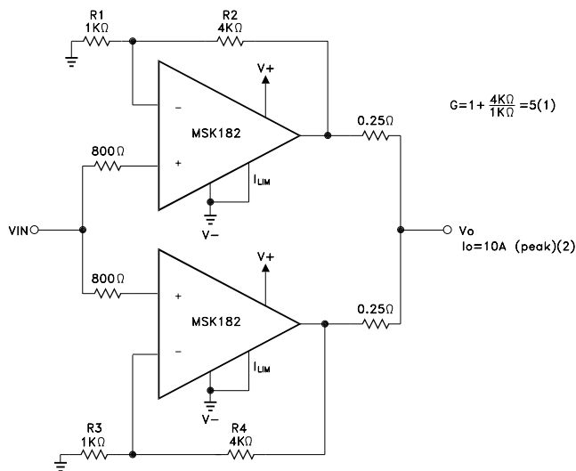
Figure 6 Parallel Output For Increased Output Current
