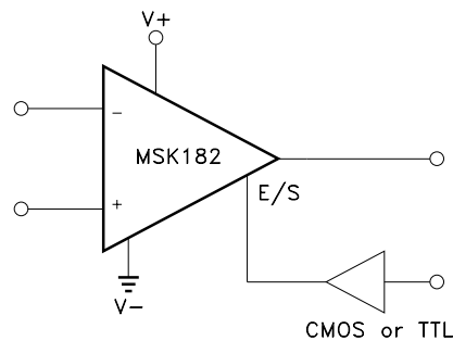
Figure 2 Output Disable with a Single Supply
