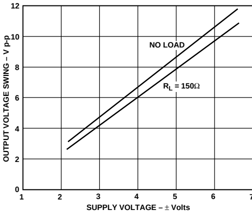
Figure 2. Output Voltage Swing vs. Supply Voltage
