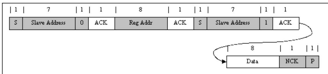
Figure 30. Single Read
