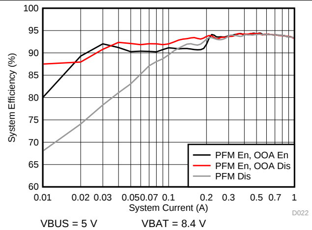
Figure 2. System Efficiency vs System Current
