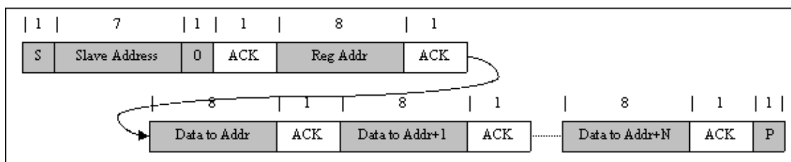
Figure 31. Multi-Write
