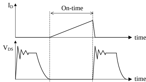
Figure 9-22 Confirmation of maximum on-time
