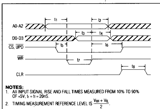
Figure 2. Timing Diagram for MX7549
