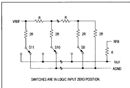
Figure 1. MX7549 Simplified DAC Schematic
