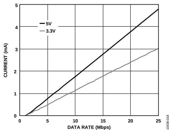
Figure 21. Typical I_{ISO(I)} Dynamic Supply Current per Input
