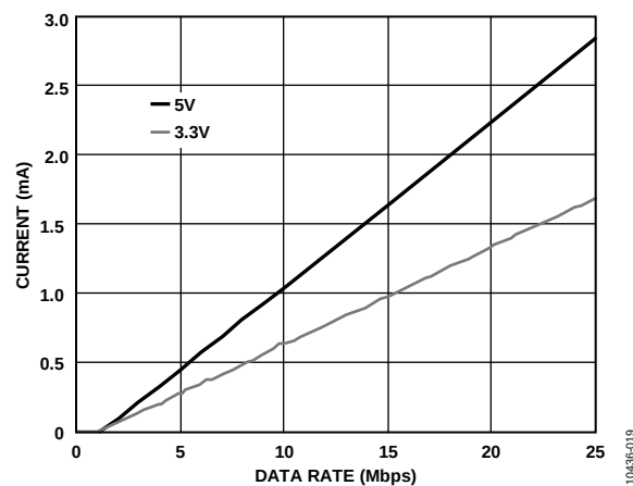
Figure 22. Typical I_{ISO(O)} Dynamic Supply Current per Output (15 pF Output Load)
