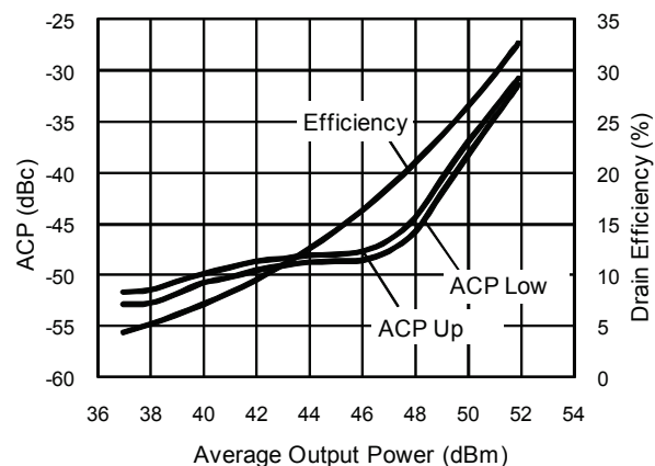
Single-carrier Drive-up, 1880 MHz V_{DD} = 30\text{ V} , I_{DQ} = 2.6\text{ A} , f = 1880\text{ MHz} , 3GPP WCDMA signal, PAR = 7.5:1, BW = 3.84 MHz
