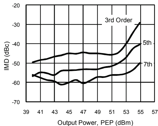
Intermodulation Distortion vs. Output Power V_{DD} = 30\text{ V} , I_{DQ} = 2.6\text{ A} , f_1 = 1880\text{ MHz} , f_2 = 1879\text{ MHz}
