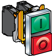
Flush push + projecting push XB4-BL845 see page 1/14
