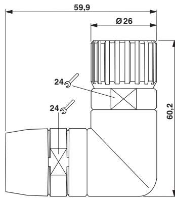
Dimensioned drawing
