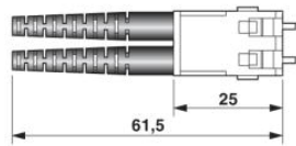
SCRJ plug connector IP20
