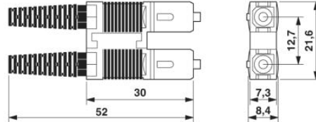
SC duplex connector IP20
