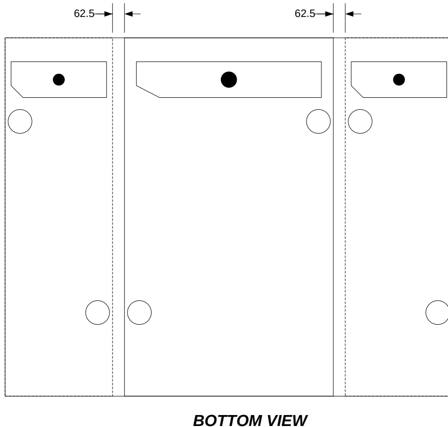
Figure 12: MDK-16 Alignment (MDK-4 and MDK-8 footprints separated by 62.5 mils)
