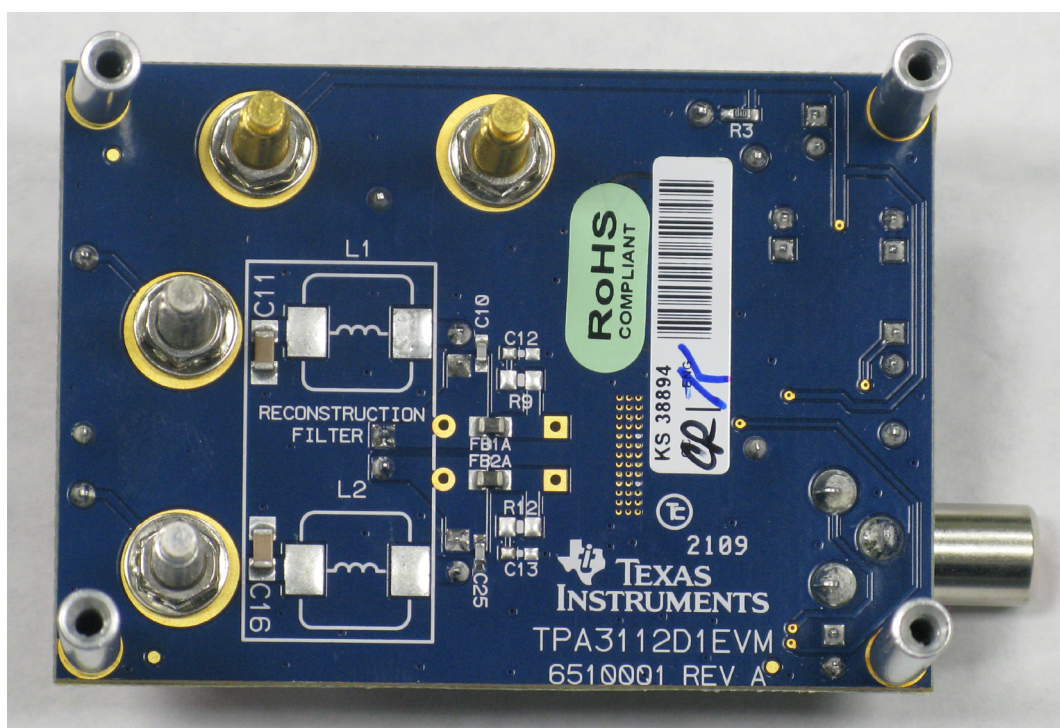
Figure 2. TI TPA3112D1EVM Audio Power Amplifier – Bottom View
