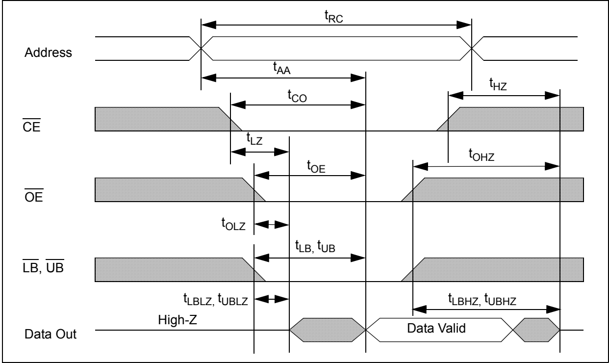
Timing Waveform of Read Cycle ( \overline{\text{WE}} = V_{\text{IH}} )
