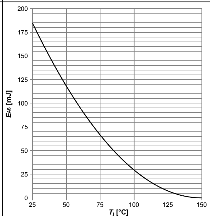
Diagram 16: Avalanche energy
