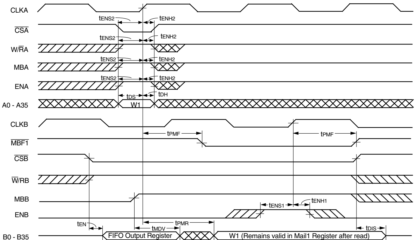
Figure 15. Timing for Mail1 Register and \overline{MBF1} Flag
